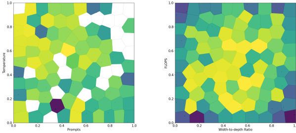
(a) Prompt archive: Prompts encoded as integers on the x -axis, normalised to be in range 0–1. On the y -axis, we have the temperature that controls LLMs exploration ability. As 1 is the maximum temperature, there is no need for normalisation. (b) Network archive: Width-to-depth ratio on the x -axis. The ratio is from 0–200 normalised to 0–1. On the y -axis, we have Float-point Operations per Second (FLOPS). We have a range of 200 Mega FLOPS to 5Giga FLOPS. This range is normalised to 0–1 for CVT-MAP-Elites.
