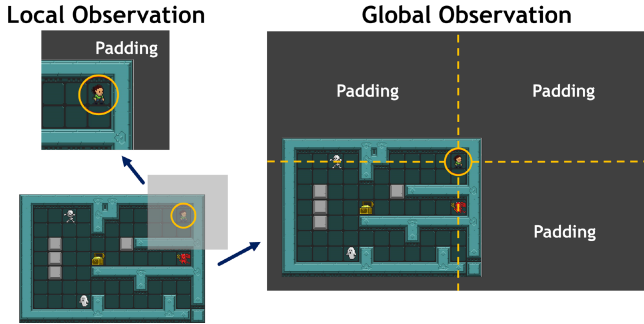
Fig. 4. Illustration of transformed game observations.
