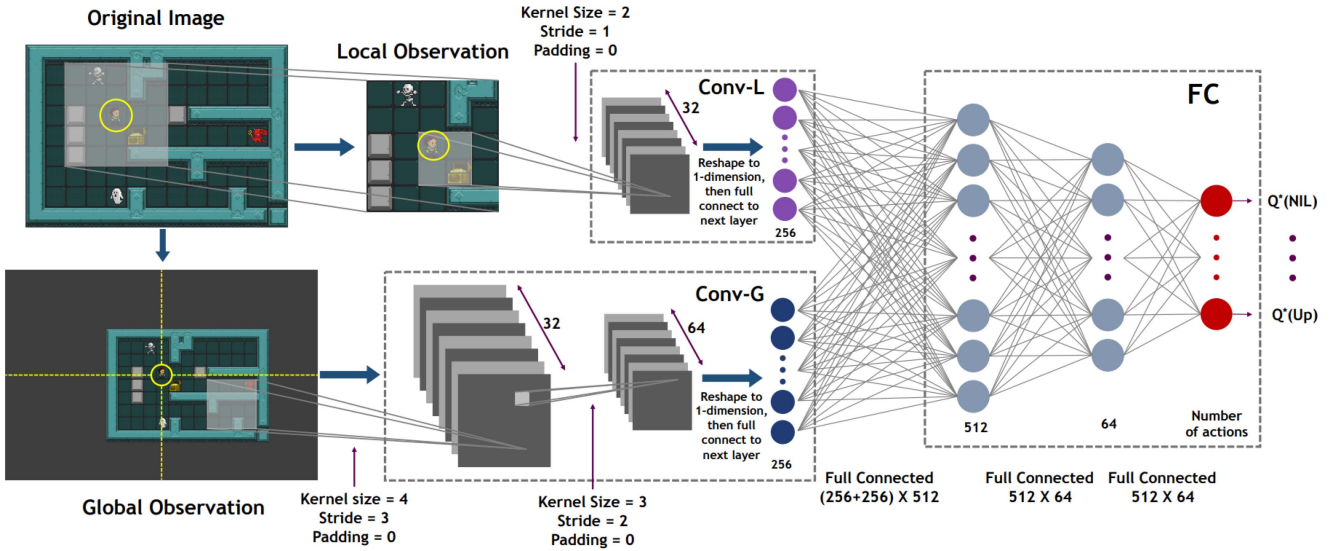
Fig. 3. Illustration of RL with dual-observation.
