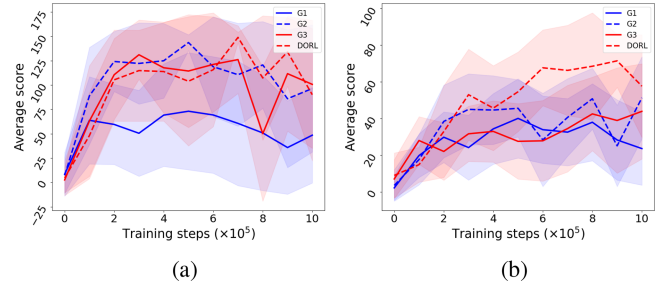
Fig. 5. Average scores obtained by PPO agents on GoldDigger 's training levels over 20 independent trials each. (a) GoldDigger-0 . (b) GoldDigger-1 .
