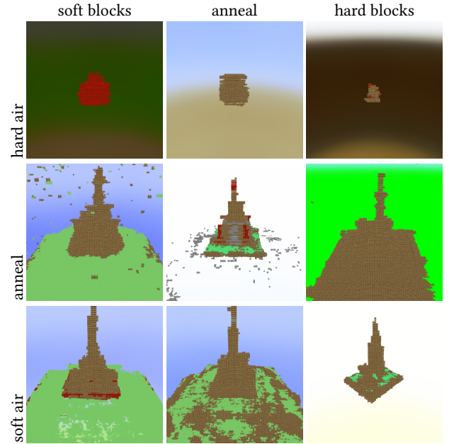
Figure 6: Qualitative Effect of Different Quantization Schemes for “dwarven entrance”. The best results obtained using hard block types and soft air blocks. Meaningful representations are learned only when the discreteness of air blocks (or by analogy, the density or topology of the generated structure) is relaxed or annealed throughout training (bottom two rows).
