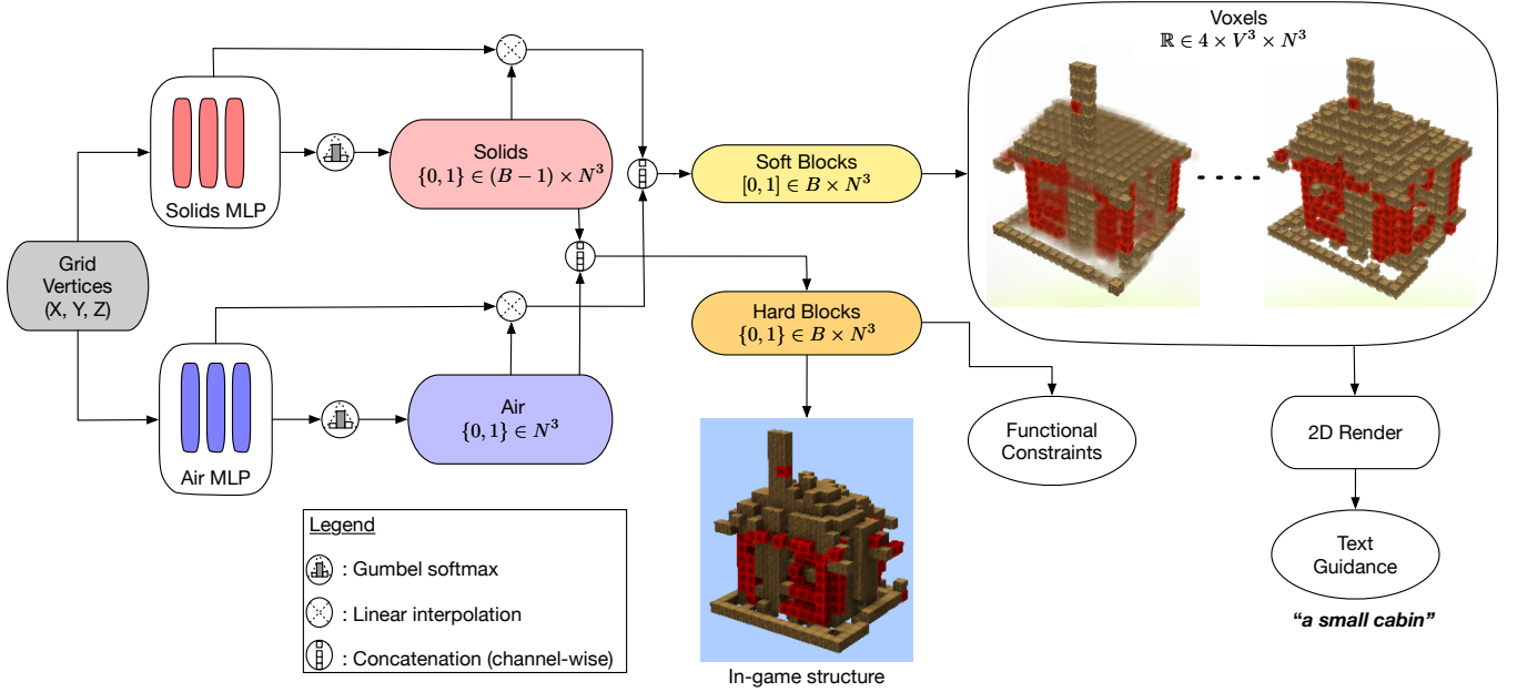
Figure 3: DREAMCRAFT produces a distribution of discrete blocks over a grid. Unquantized or “soft” versions of this distribution can be visualized for text-image guidance, while a fully discrete representation can be used to determine functional constraints, and exported to an in-game structure.
