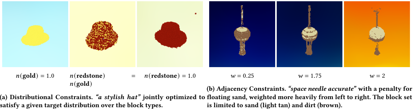
Figure 7: Examples of incorporation of functional constraints via auxiliary loss terms.
