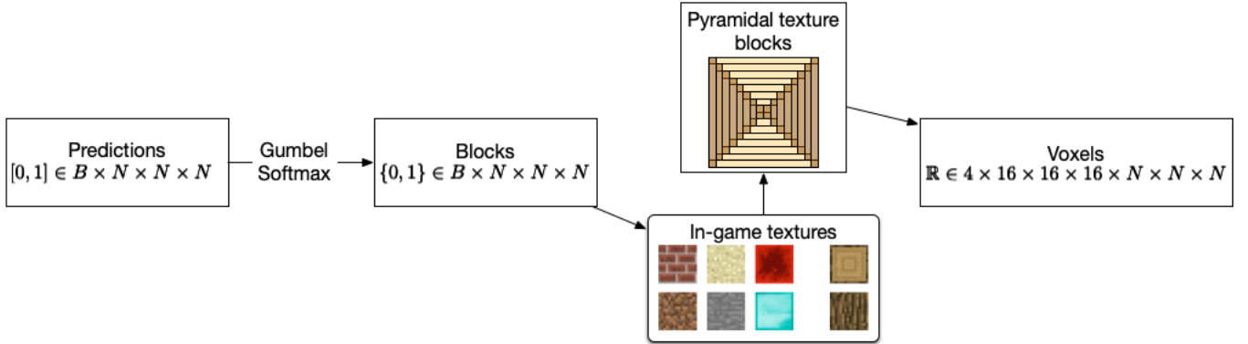
Figure 4: From 2D textures to 3D structures Once discretized, block types are mapped to voxel grids corresponding to the appearance of objects in-game. Here, we assemble each block into a 3D voxel grid using 2D textures from Minecraft. We approximate solid blocks by repeating the surface texture in the space inside the block.
