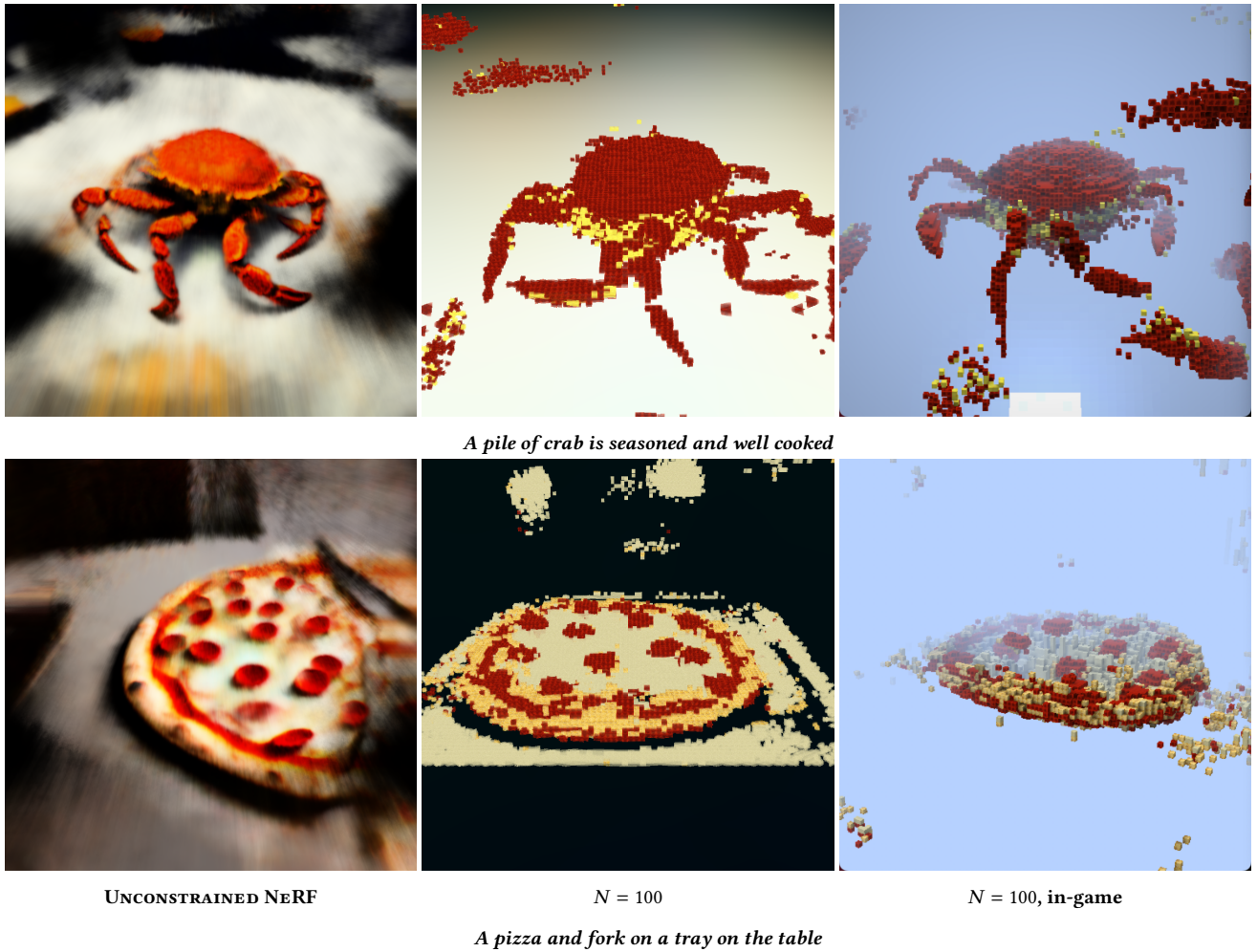
Figure 8: DREAMCRAFT output given COCO dataset captions, viewed in-game (right), by neural rendering (middle), and standard text-guided NeRF output (left) given the same prompts.
